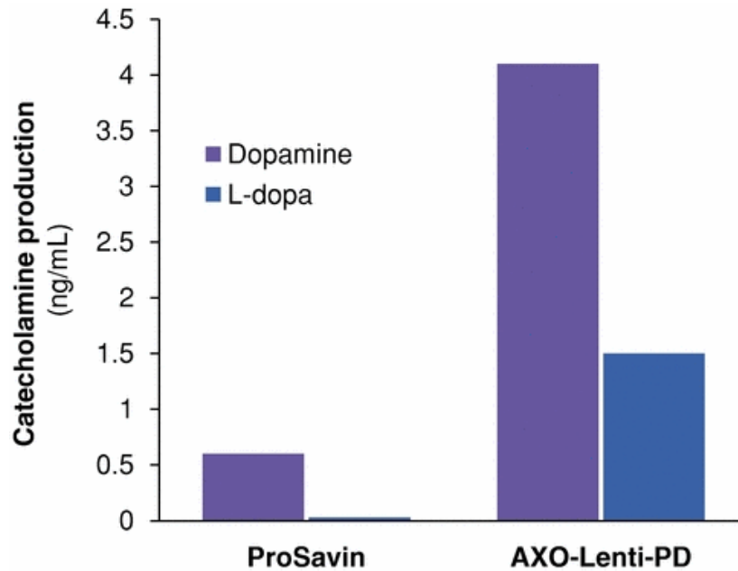
Comparison of Catecholamine (L-dopa and Dopamine) Production Between ProSavin and AXO-Lenti-PD in Primary Human Cortical Neurons
