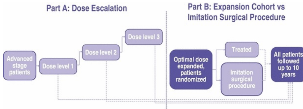
Flow Diagram of Planned Phase 1/2 Clinical Trial of AXO-Lenti-PD
